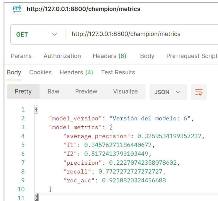
FIGURA 4.8. Champion - metrics
