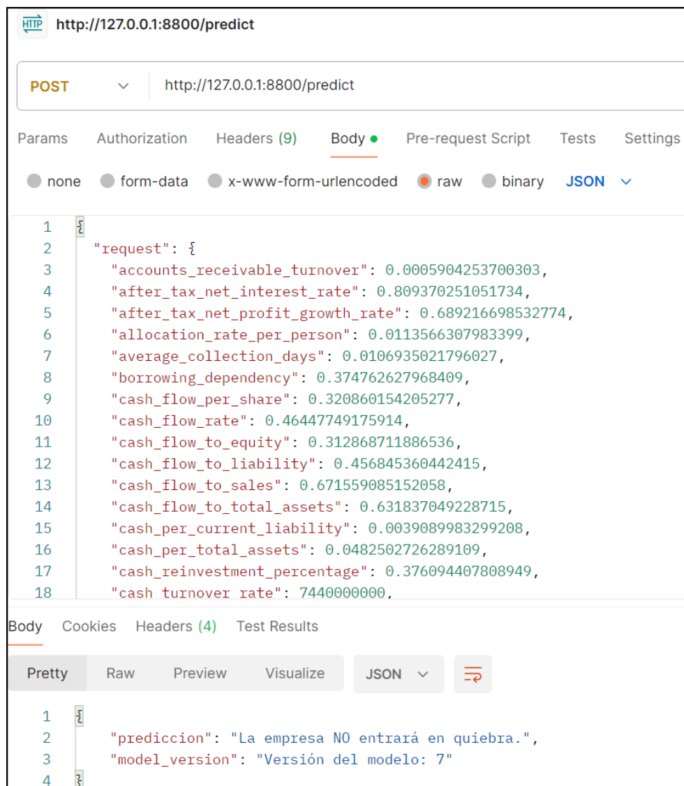
FIGURA 4.9. Endpoint predict
